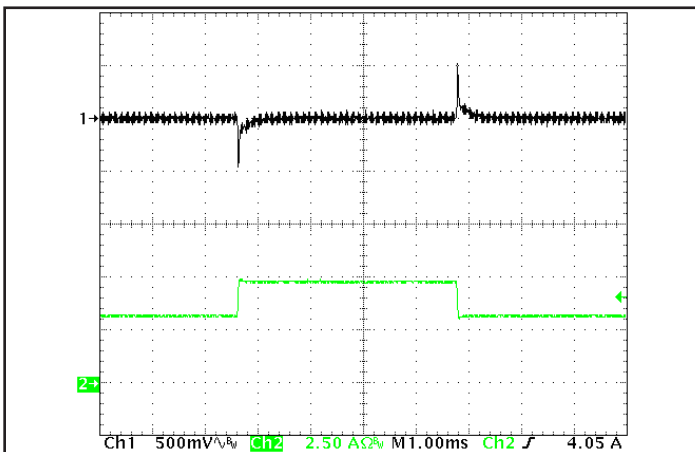
Figure 5: Output voltage response to step-change in load current (50% -75% -50% of I_{out(max)} ; dI/dt = 0.2 A/\mu s ). Load cap: 1 \mu F ceramic and 15 \mu F tantalum capacitors. Ch 1: V_{out} , Ch 2: I_{out} .
